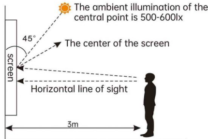
Figure 1 side view
