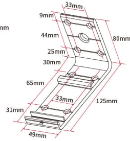
Wall bracket
