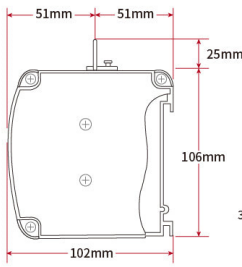
Side view of case
