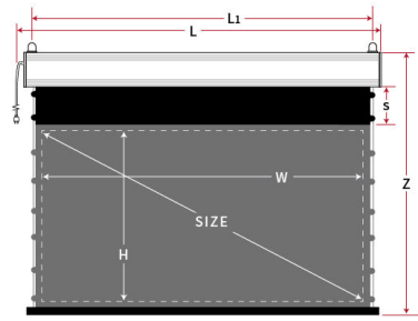
Front view of screen (The actual standard view area is within the dotted line)
